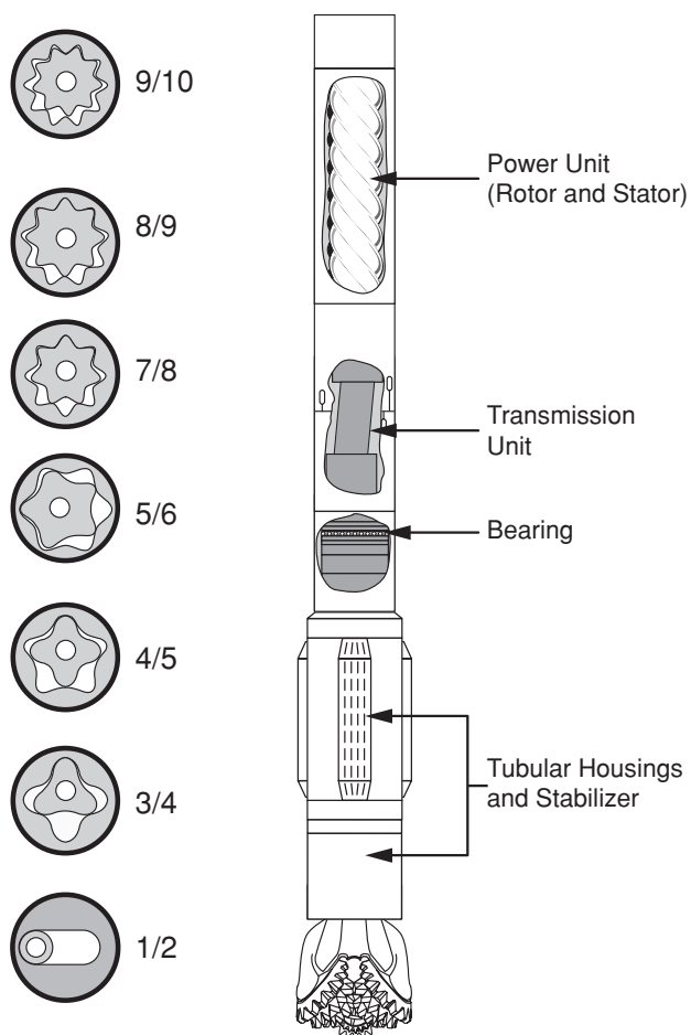
Figure 14 PDM assembly
