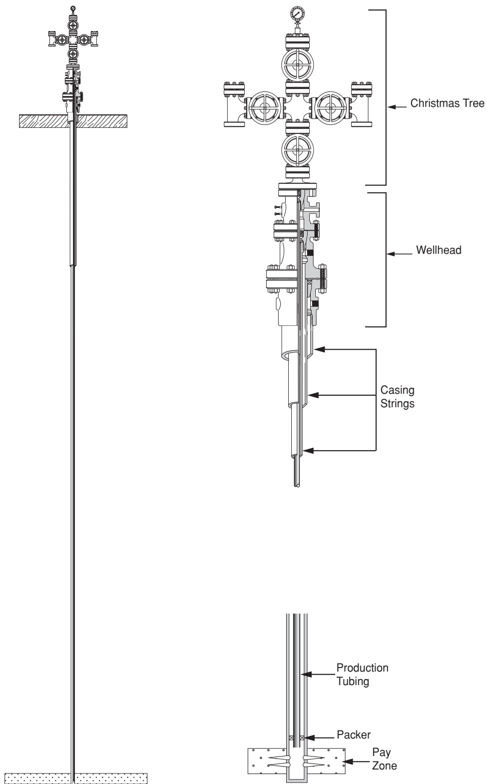
Figure 5 Completion schematic
