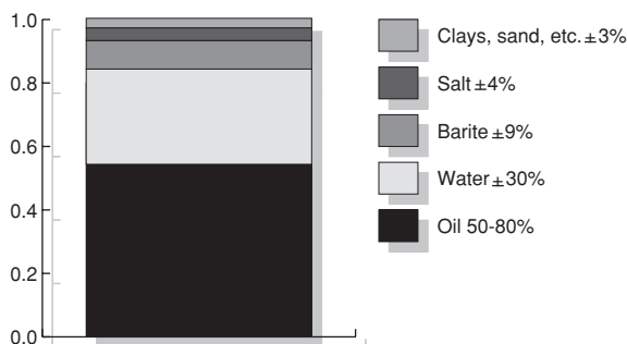
Figure 3 Composition of typical oil-based mud
