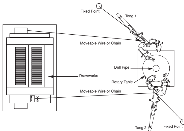
Figure 10 Tubing makeup and breakout
