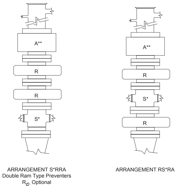
Figure 32 (b) Normal pressure stack
