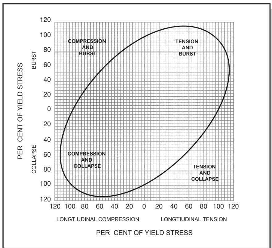
Figure 18 Tri-axial loading ellipse
