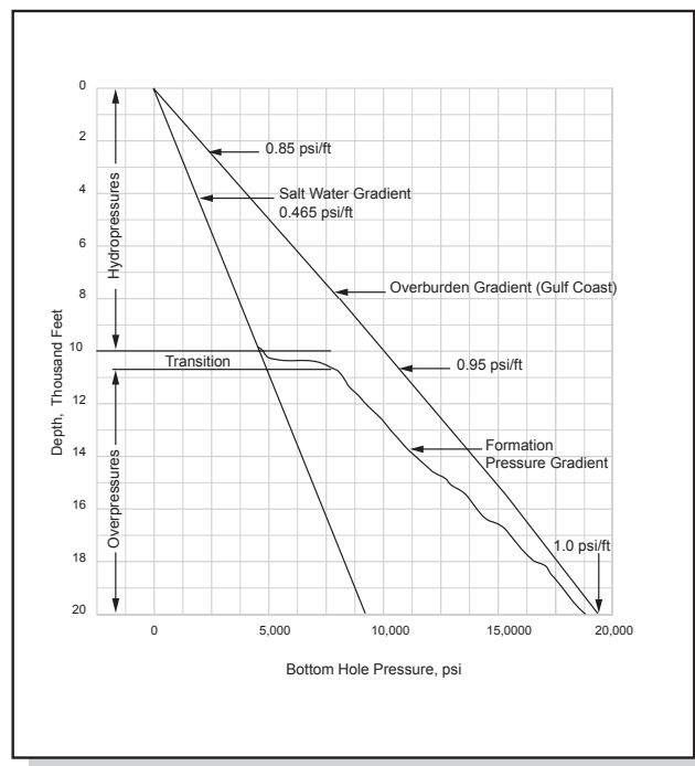
Figure 13 Transition from normal pressures to overpressures
