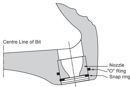
Figure 15 Jet nozzles
