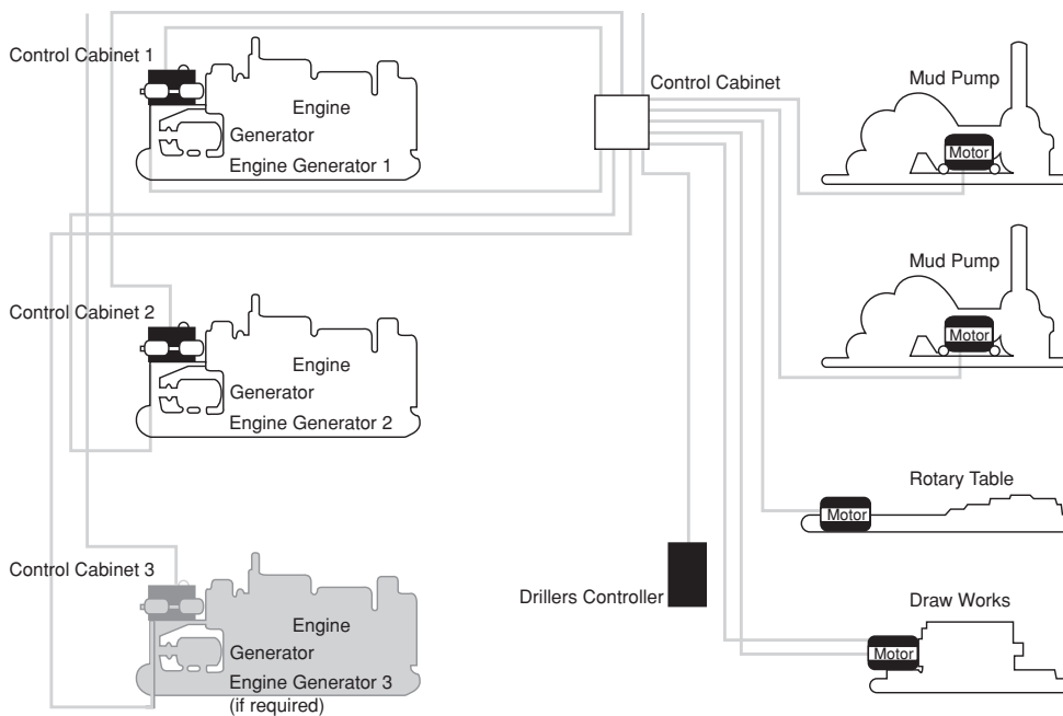
Figure 2 Power system
