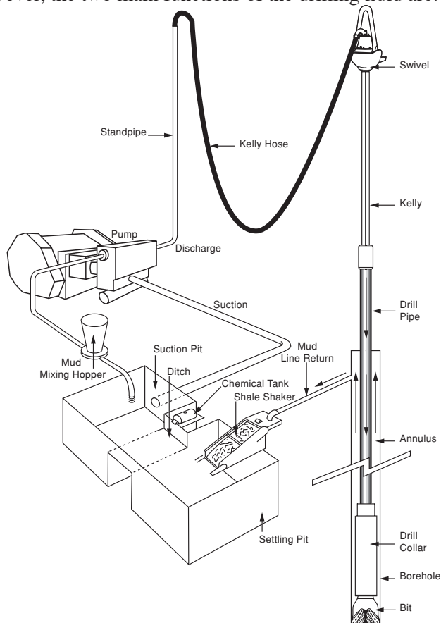
Figure 6 Circulating system
