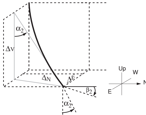
Figure 3 Tangential Model
