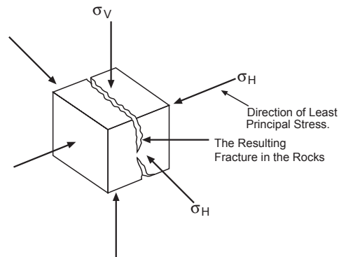
Figure 20 Idealised view of the stresses acting on the block
