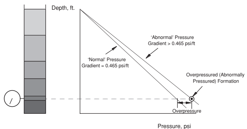
Figure 5 Overpressured Formation
