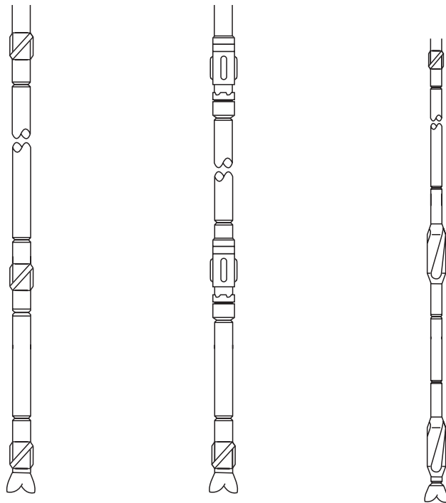
Figure 14 Typical BHA's
