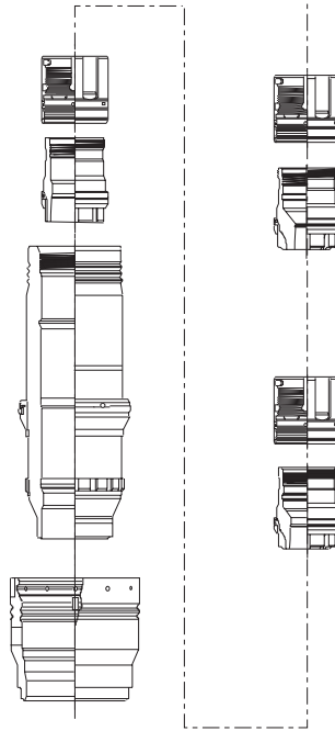
Figure 2 Casing Configuration
