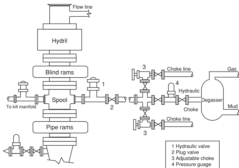
Figure 16 BOP stackup
