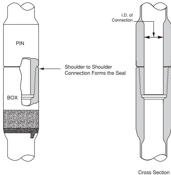
Figure 4 Tool joint
