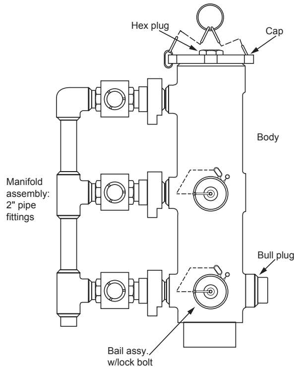
Figure 9 Cement Head
