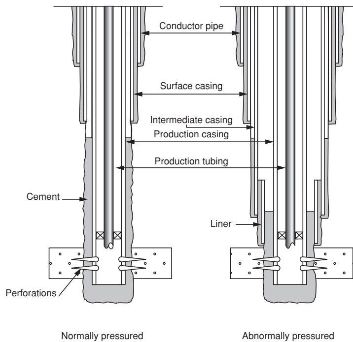
Figure 1 Functions of Primary Cementing
